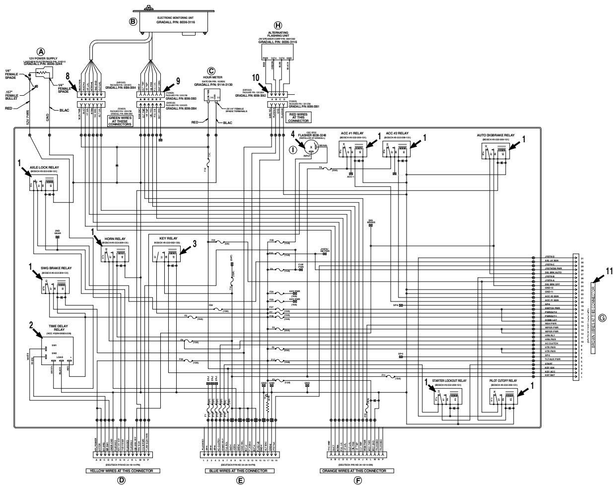
Figure 10-2 Circuit Board
