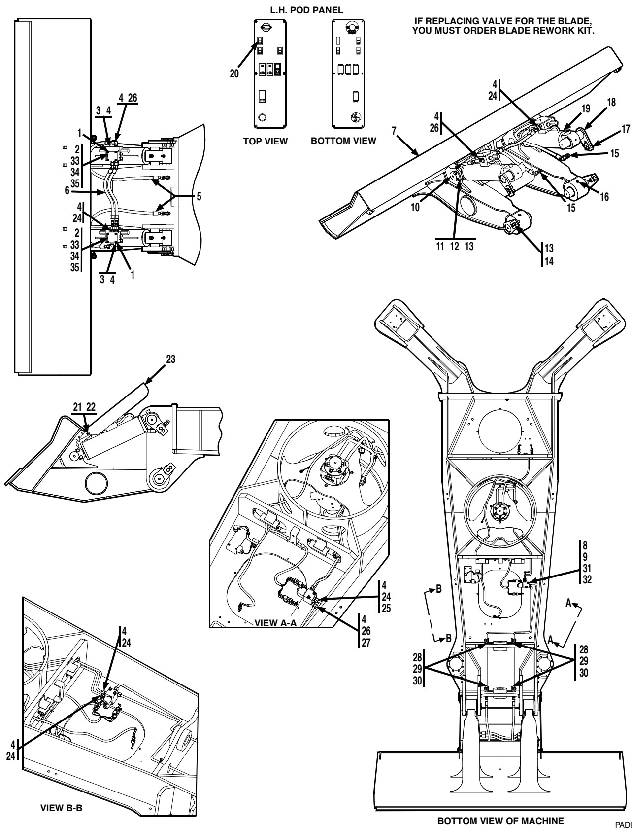
Figure 12-10 Chassis Mounted Blade Installation Components
