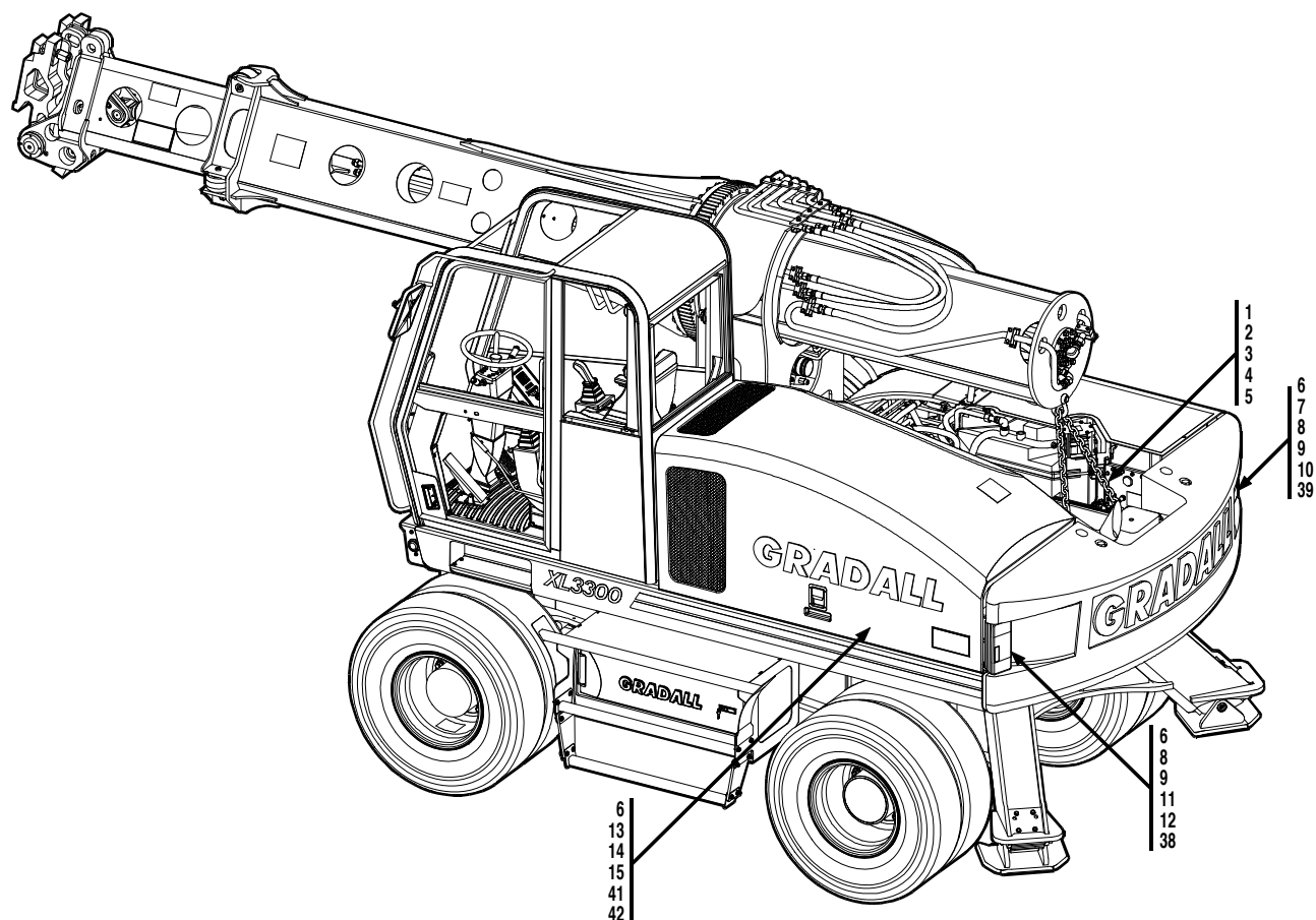
Figure 1-4 R.H. Rotating Platform
