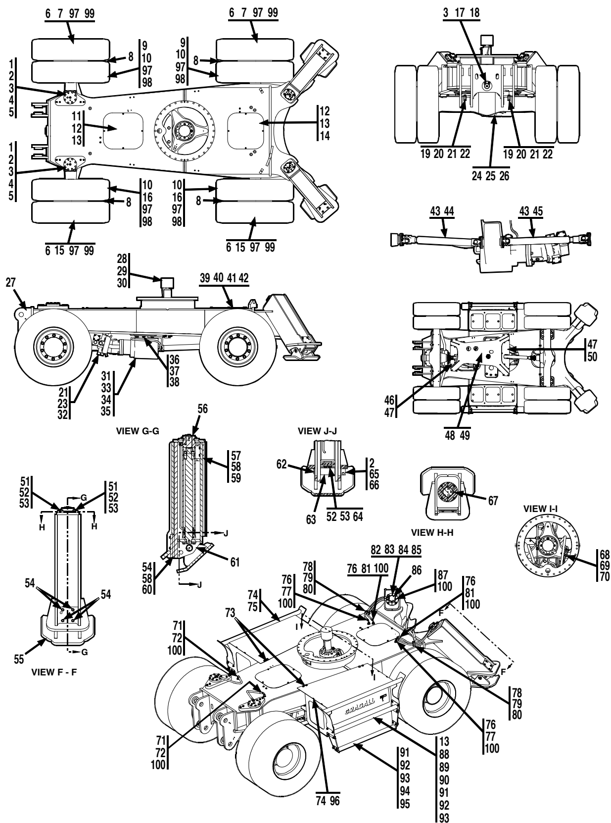
Figure 1-1 Frame Assembly
