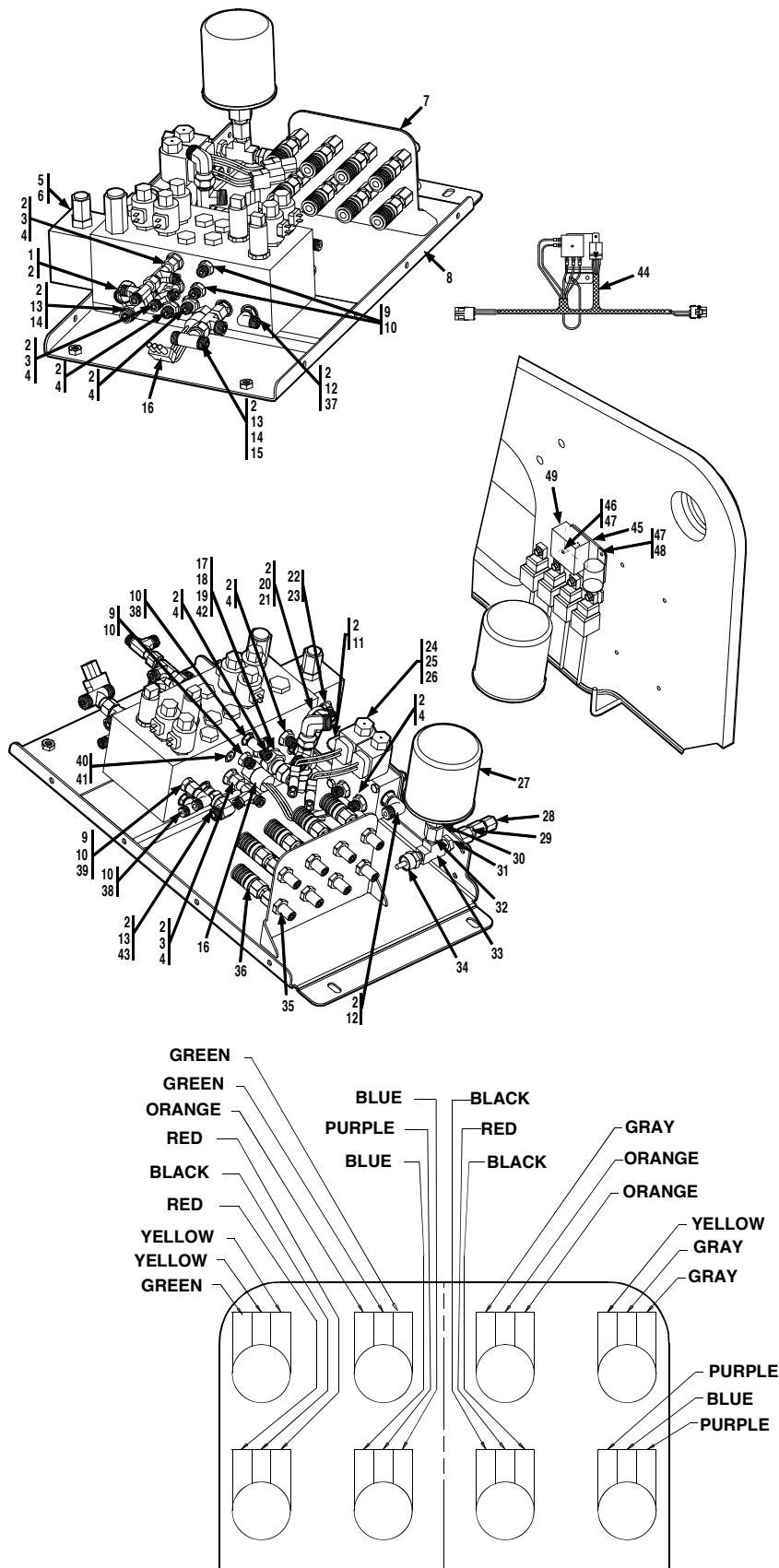
Figure 9-10 Pilot Manifold Valve Tray Hydraulic Components
