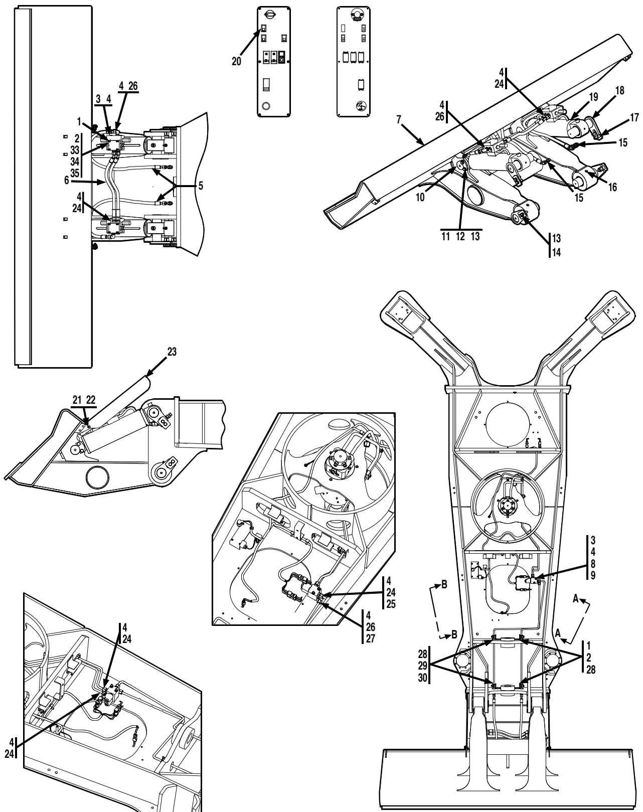
Figure 12-10 Chassis Mounted Blade Installation Components
