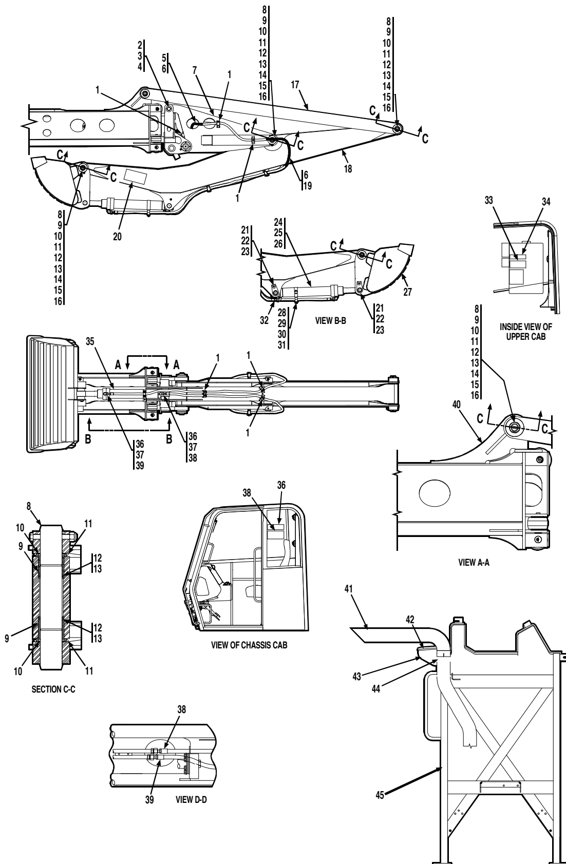
Figure 3-9 Telestick Adapter Installation
