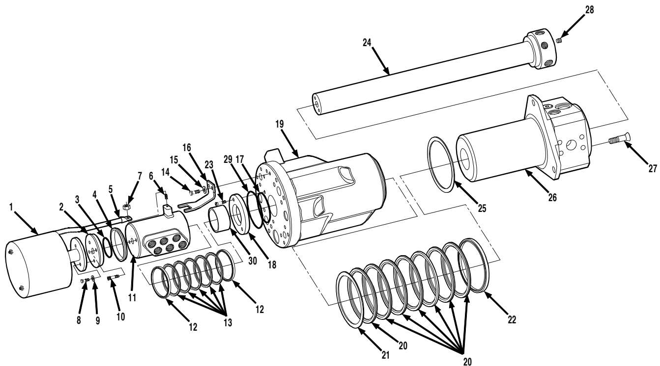
Figure 9-28 Center Pin
