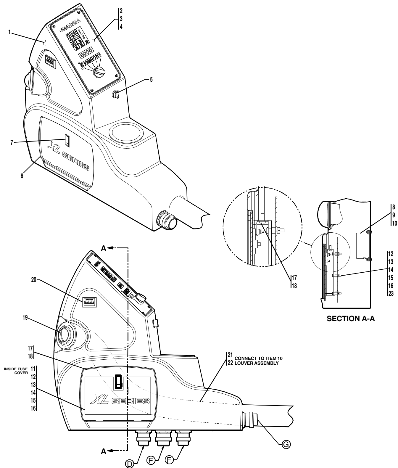
Figure 6-5 Cab Console
