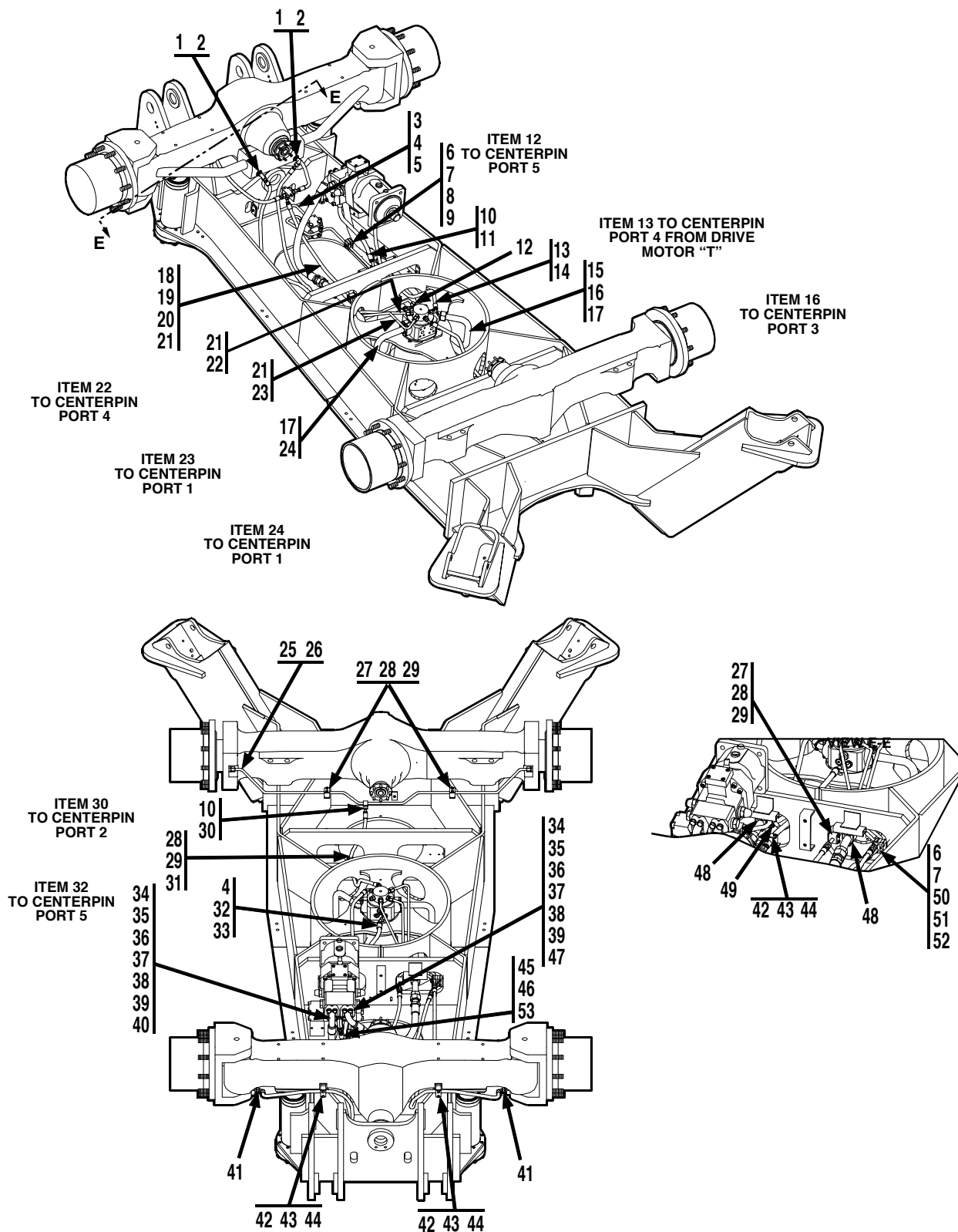
Figure 1-2 Frame & Plumbing
