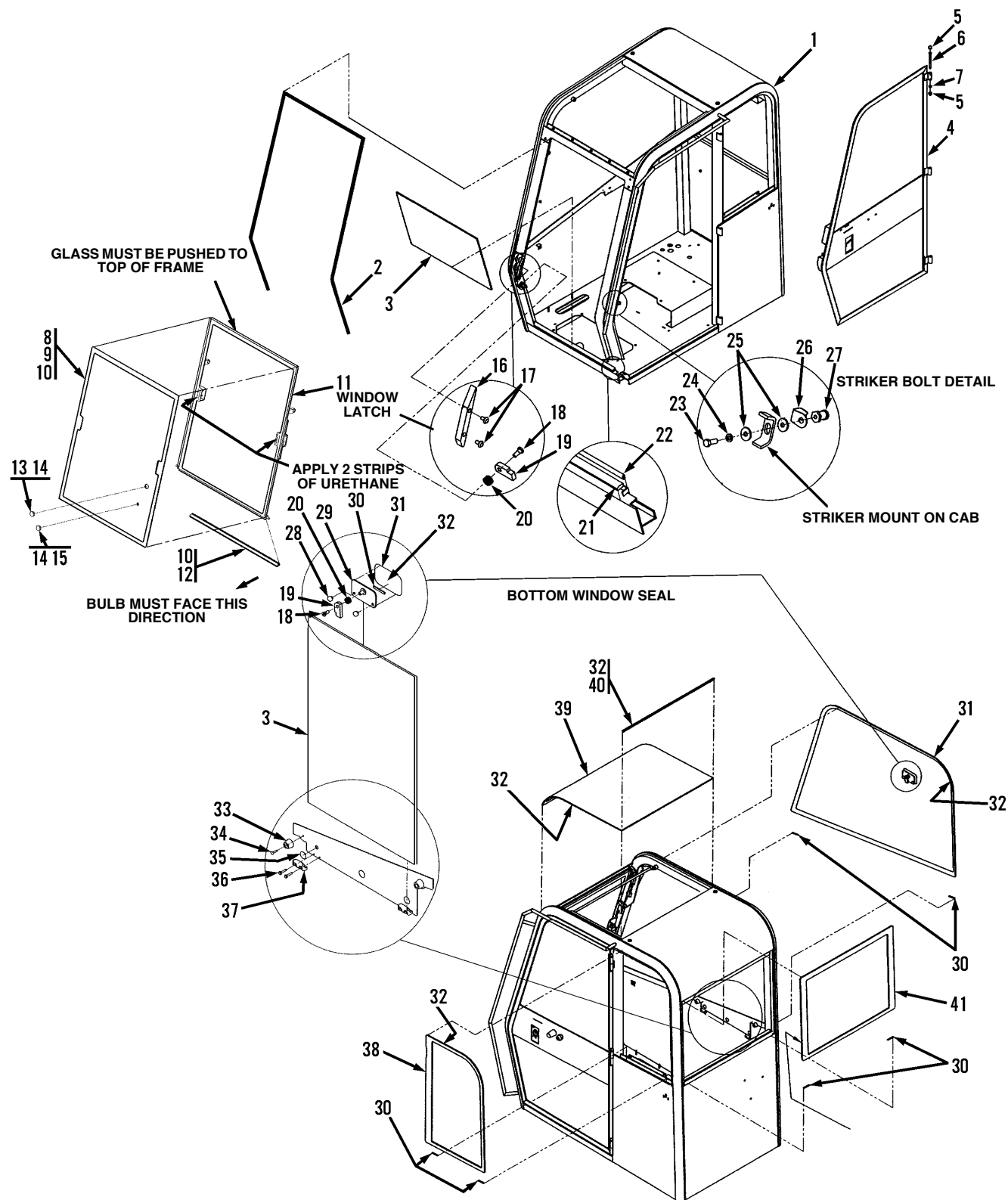
Figure 6-1 Operators Cab
