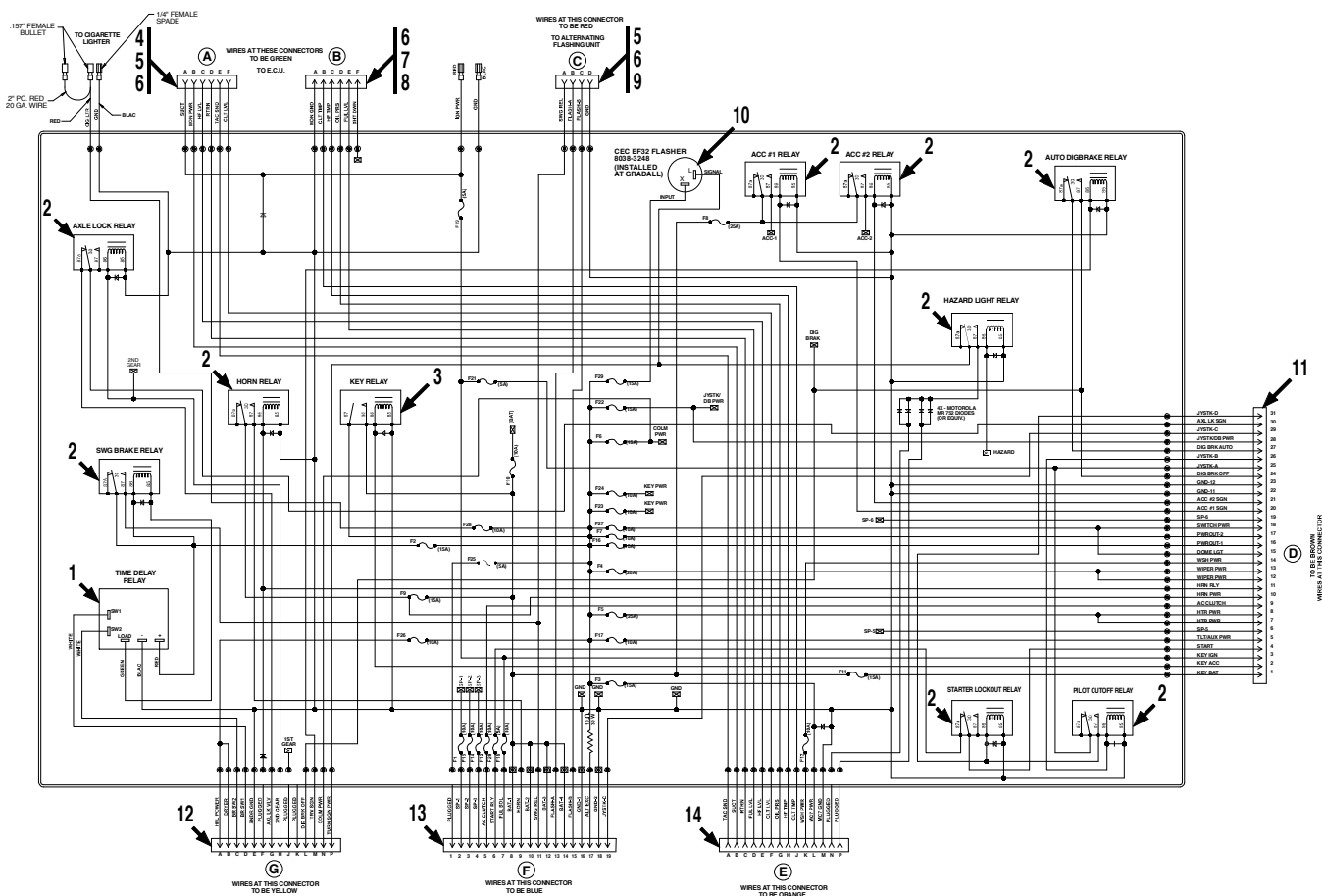
Figure 10-2 Circuit Board
