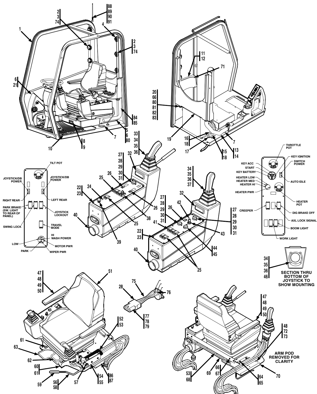
Figure 6-4 Cab Interior Components
