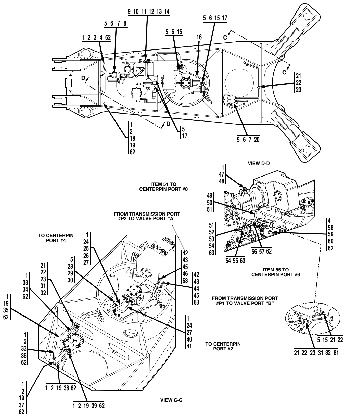
Figure 1-2 Frame & Plumbing
