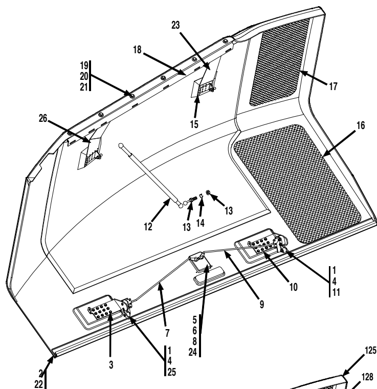
Figure 1-6 Engine Cover
