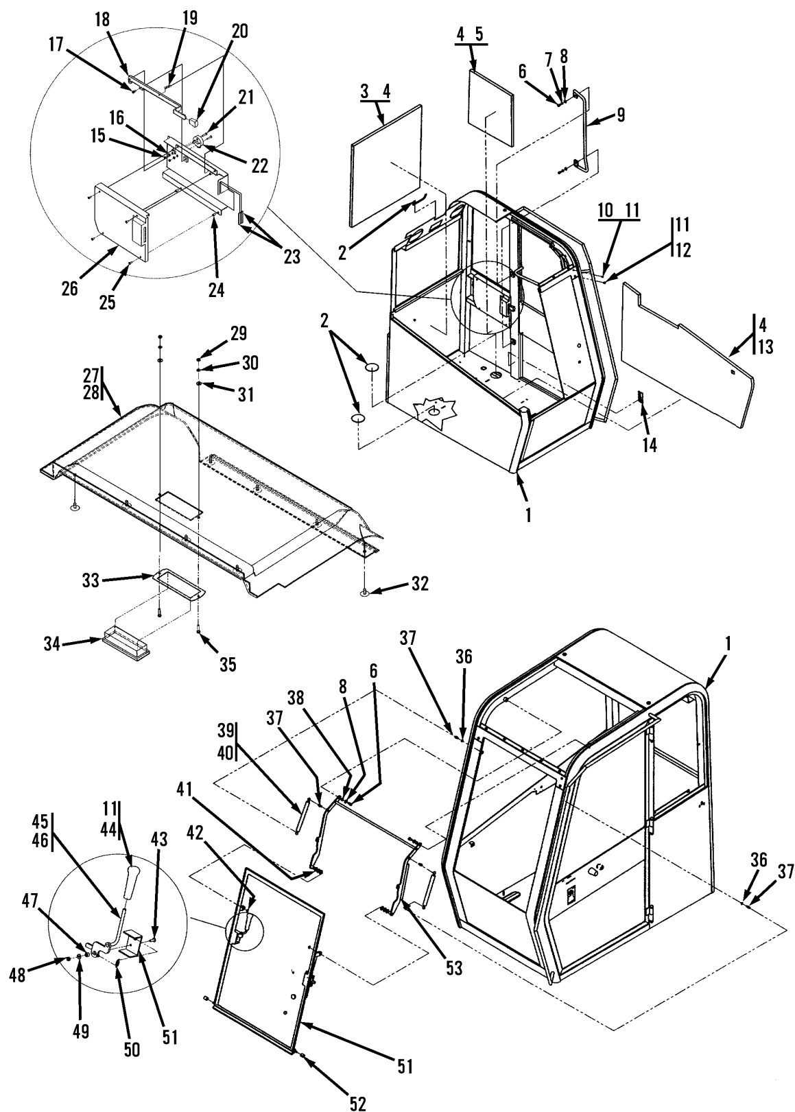
Figure 6-2 Operators Cab
