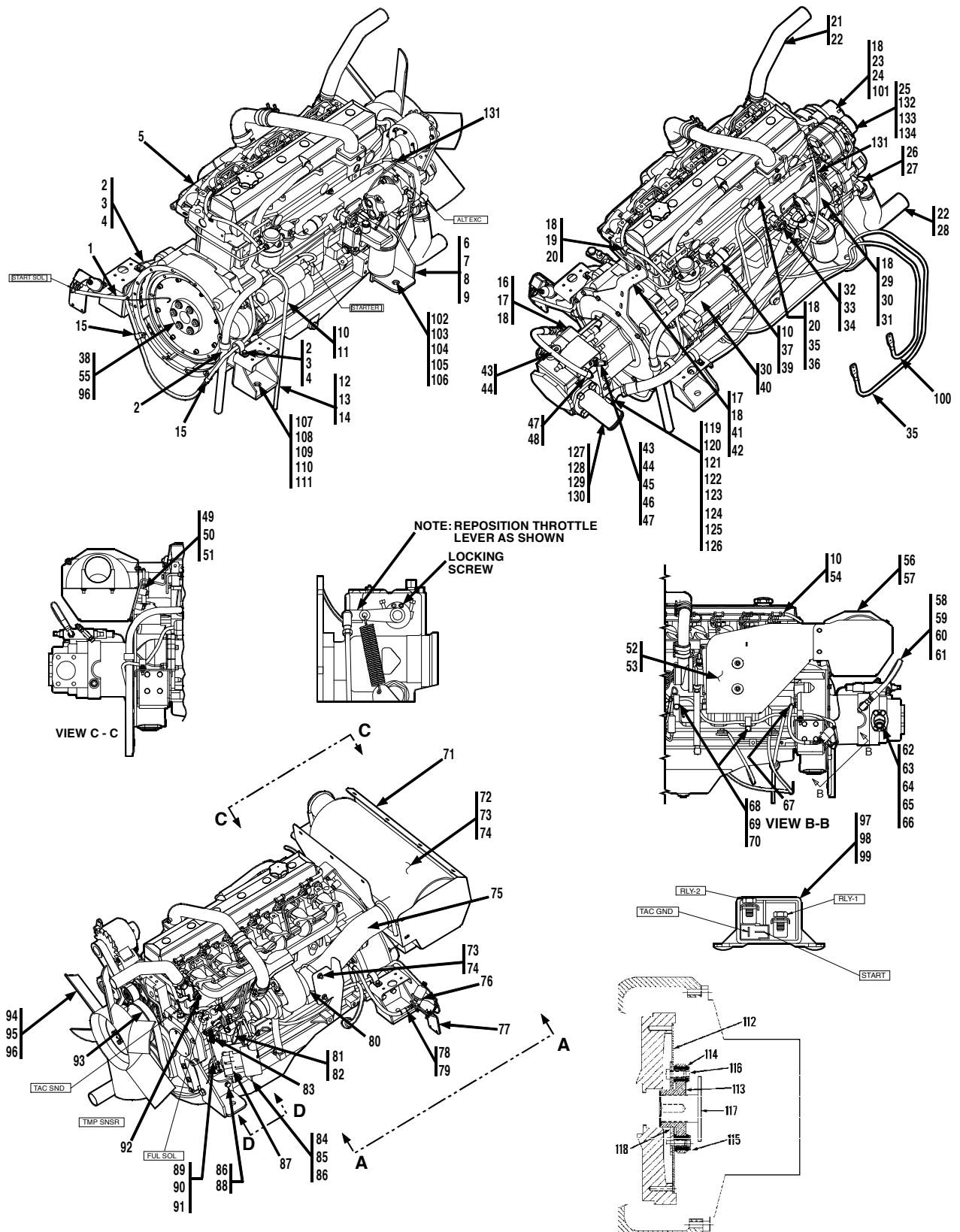
Figure 4-1 Engine Assembly
