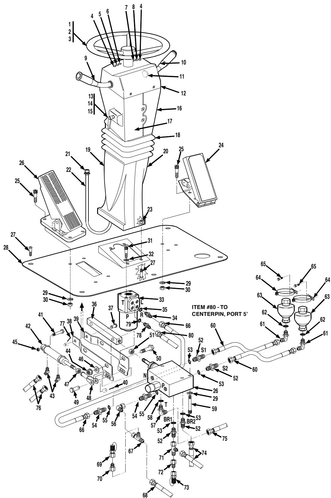
Figure 7-2 Steering Column, Foot Pedals & Installation
