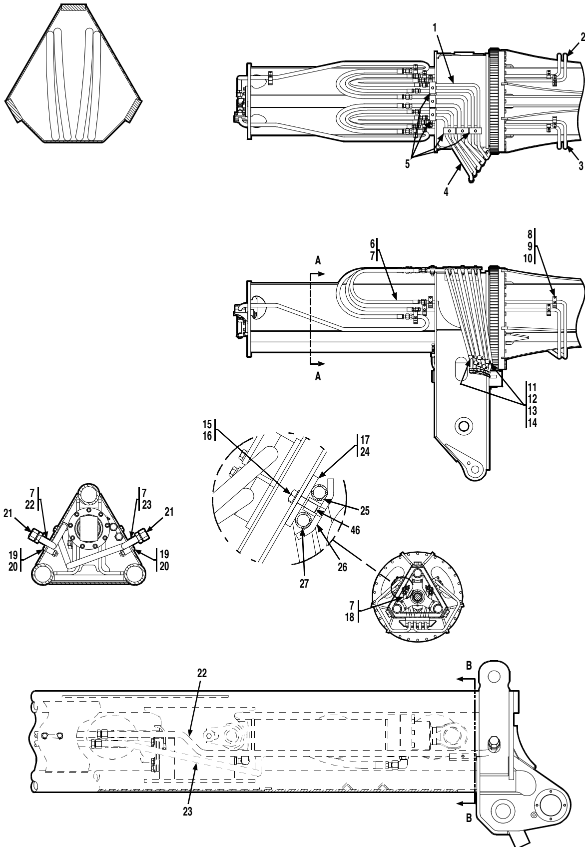
Figure 12-14 Auxiliary Hydraulic Field Installation Components
