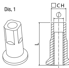
nipple design
